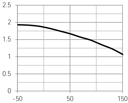
Fig.3 Threshold Voltage V.S Junction Temperature
