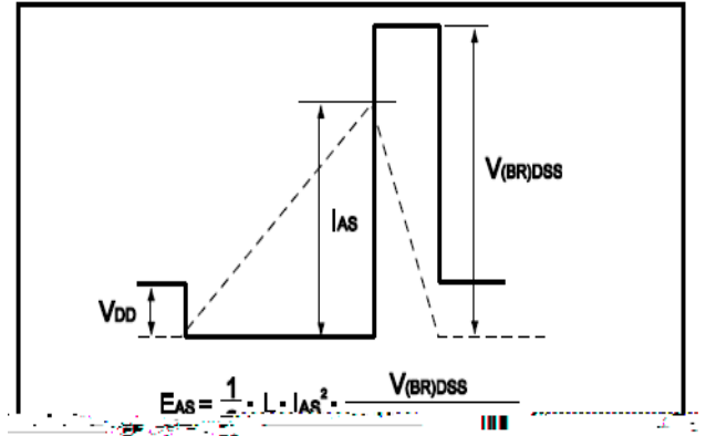
Fig.6 Avalanche Waveform
