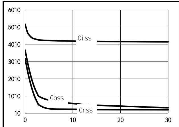
Fig.2 Capacitance Characteristics
